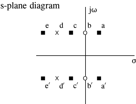
FIGURE 32-4 Pole-zero example. The notch filter has two poles (represented by x) and two zeros (represented by o). This s -plane diagram shows the five locations we will "probe" in this example to analyze this system. (Figure 32-5 is a continuation of this example).
