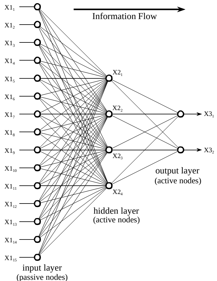
FIGURE 26-5 Neural network architecture. This is the most common structure for neural networks: three layers with full inter-connection. The input layer nodes are passive, doing nothing but relaying the values from their single input to their multiple outputs. In comparison, the nodes of the hidden and output layers are active, modifying the signals in accordance with Fig. 26-6. The action of this neural network is determined by the weights applied in the hidden and output nodes.
