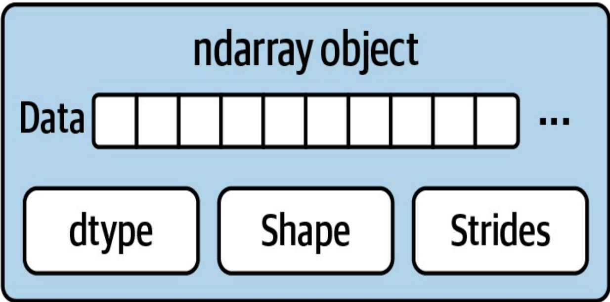
Figure A-1. The NumPy ndarray object
